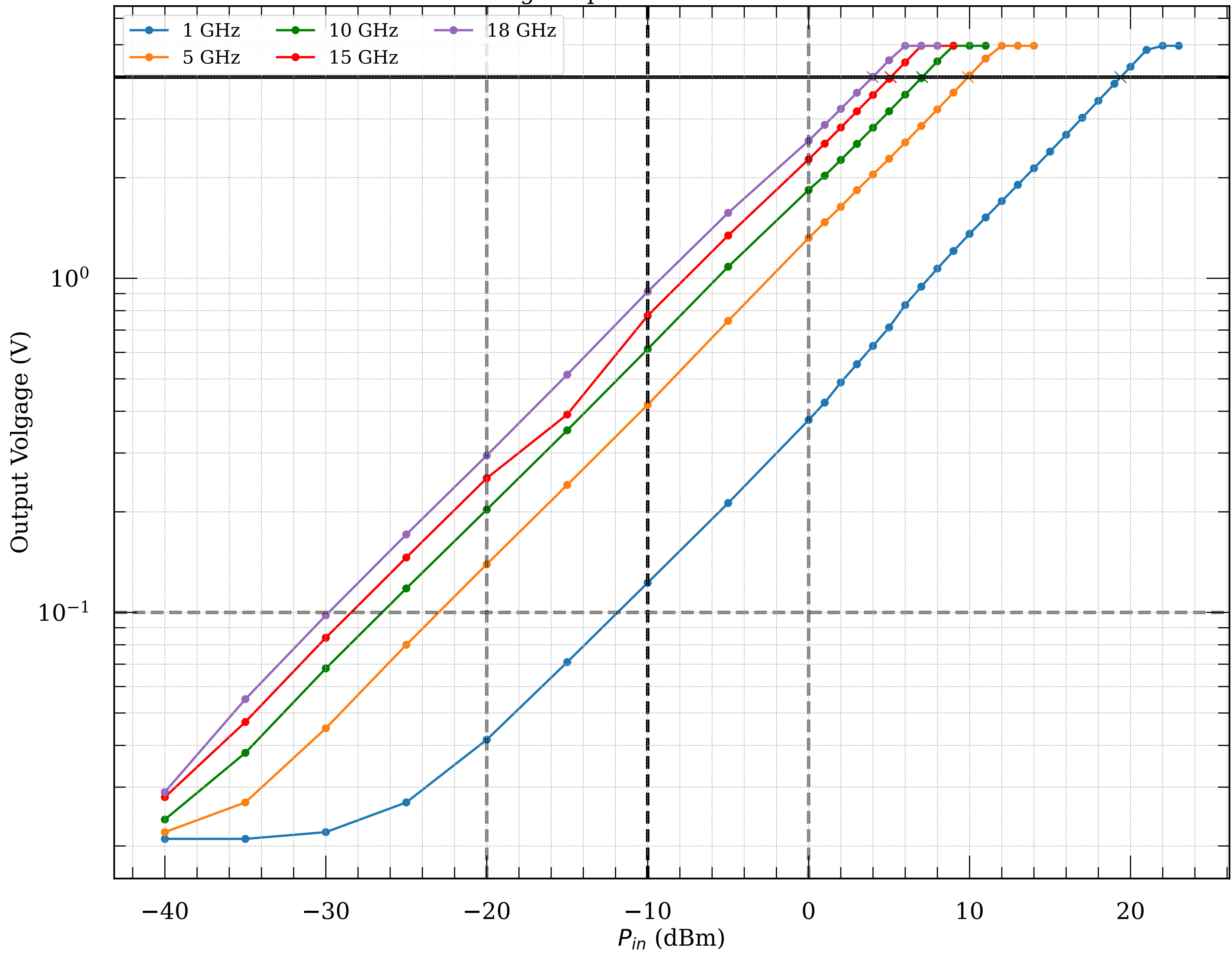
Measured voltage-to-power curve of detector module028
